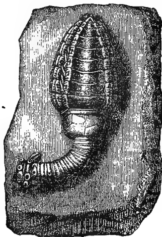
CUPRESSOCRINUS CRASSUS. (Old Red Sandstone.)
